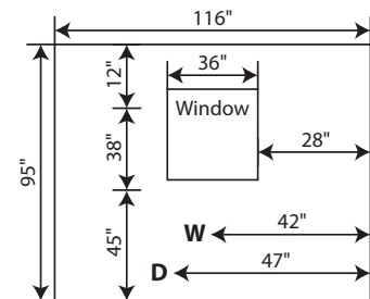
Example 2, Elevation
